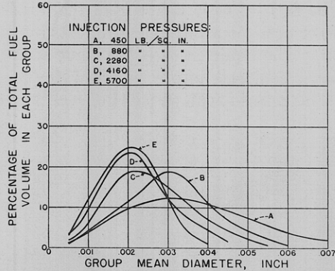
FIG. 4. Effect of jet velocity on atomization
