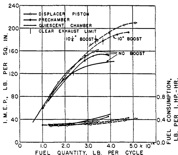
FIG. 14. Performance with typical combustion chambers
