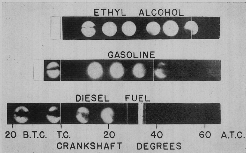
FIG. 10. Vaporization and condensation of fuel. Engine R. P. M. = 1500; I. A. A. = 20^{\circ}
