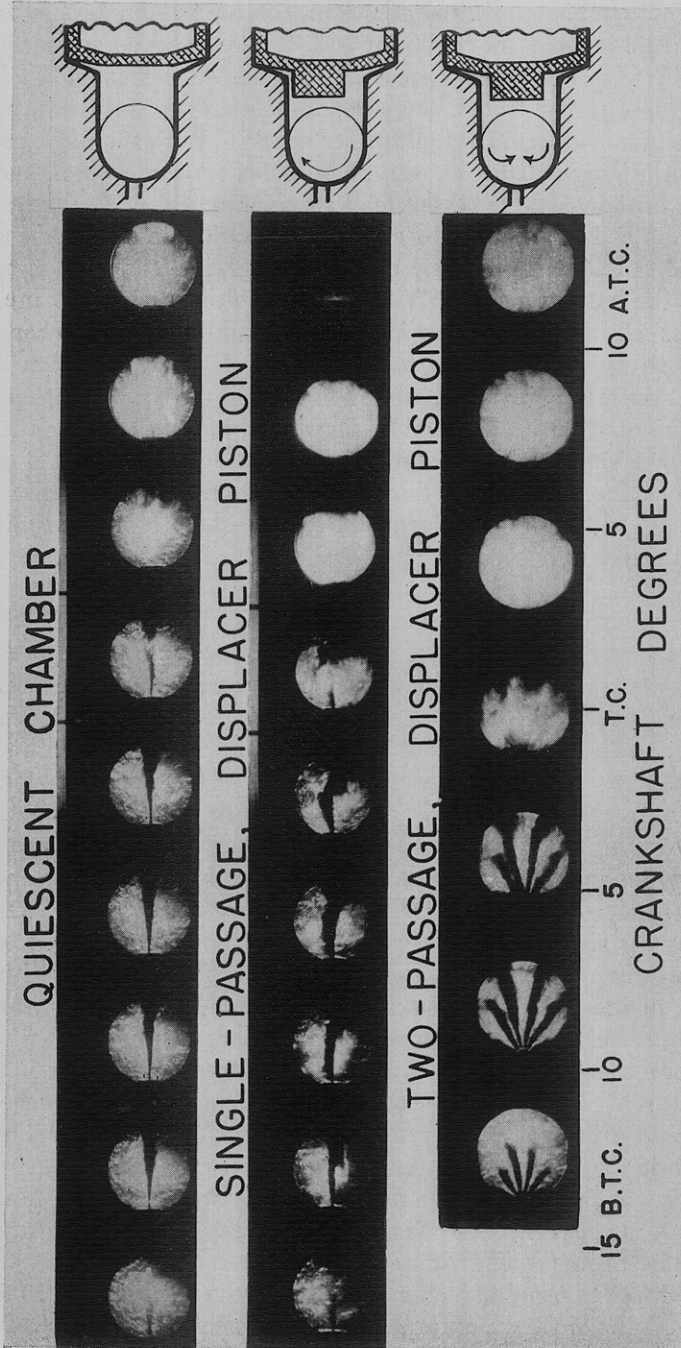
FIG. 12. Effect of air flow on fuel sprays. Engine R. P. M. = 1500; I. A. A. = 15° to 20°
